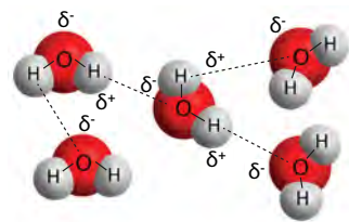
Figure 2.11. Hydrogen bonding.
